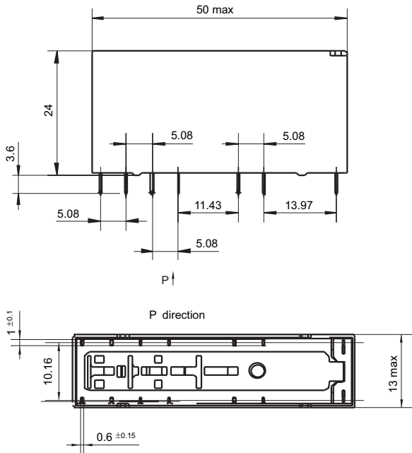
Outline Dimensions
